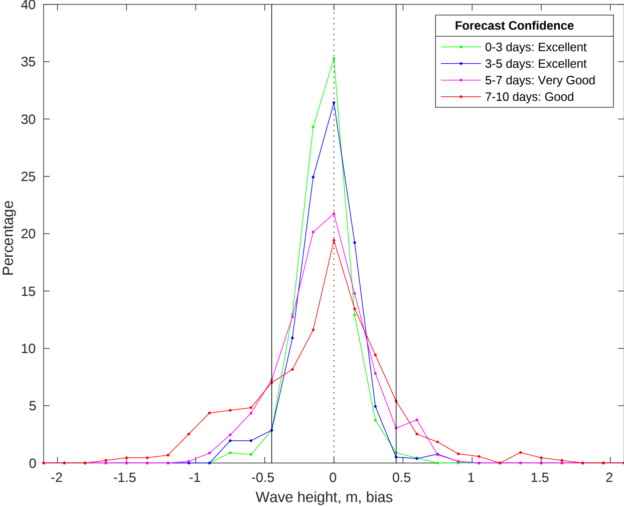
NDBC 46054 vs CMEMS Waves Bias Histogram: 17-Oct-2025
