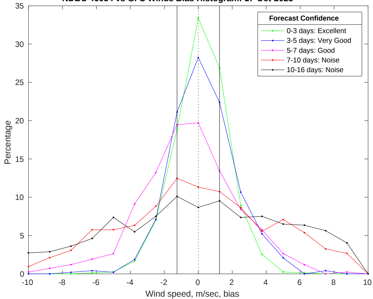
NDBC 46054 vs GFS Winds Bias Histogram: 17-Oct-2025
