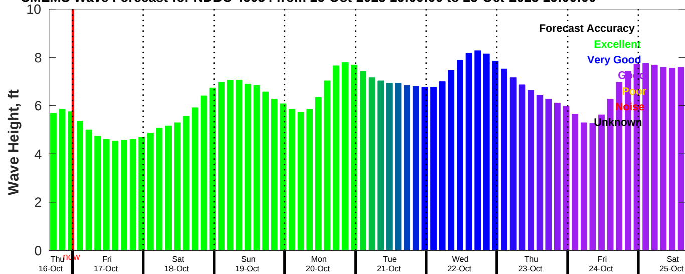
CMEMS Wave Forecast for NDBC 46054 from 16-Oct-2025 16:00:00 to 25-Oct-2025 16:00:00
