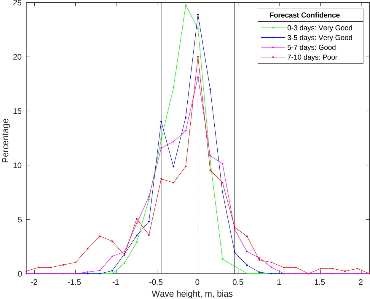
NDBC 46069 vs CMEMS Waves Bias Histogram: 17-Oct-2025
