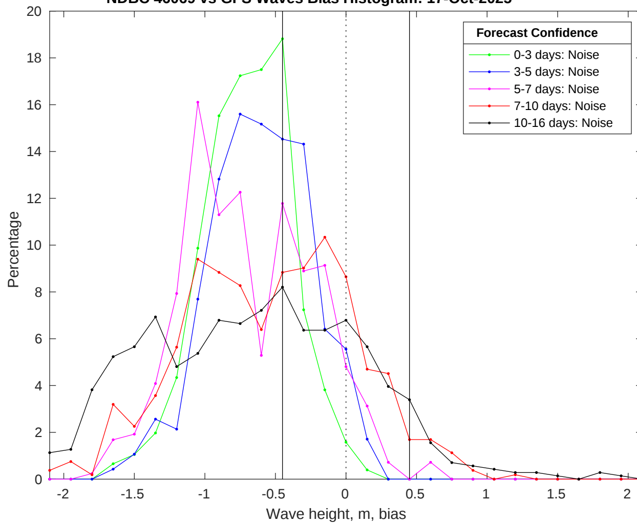
NDBC 46069 vs GFS Waves Bias Histogram: 17-Oct-2025
