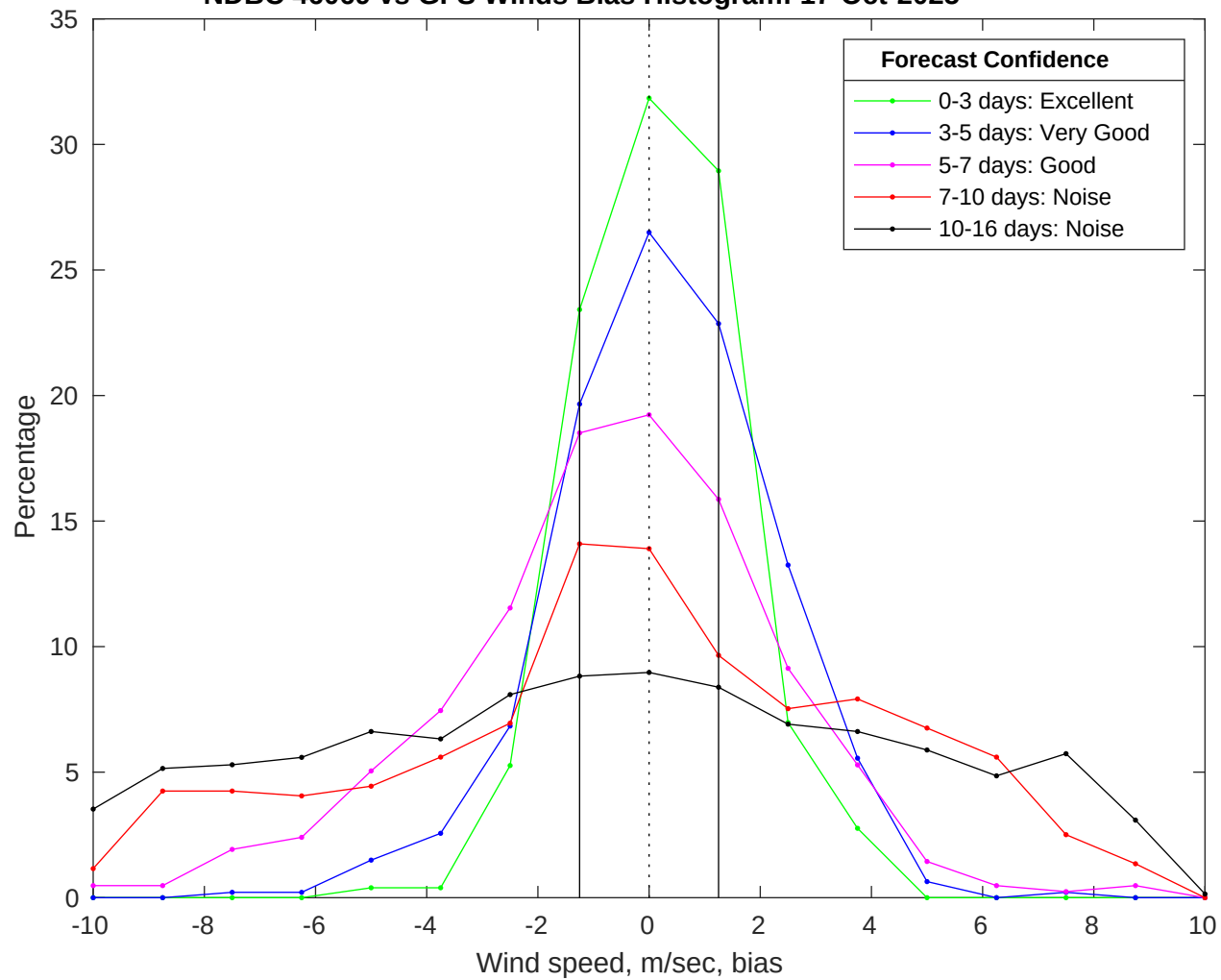
NDBC 46069 vs GFS Winds Bias Histogram: 17-Oct-2025
