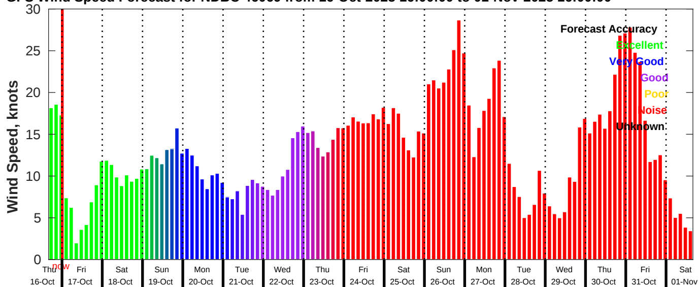
GFS Wind Speed Forecast for NDBC 46069 from 16-Oct-2025 16:00:00 to 01-Nov-2025 16:00:00
