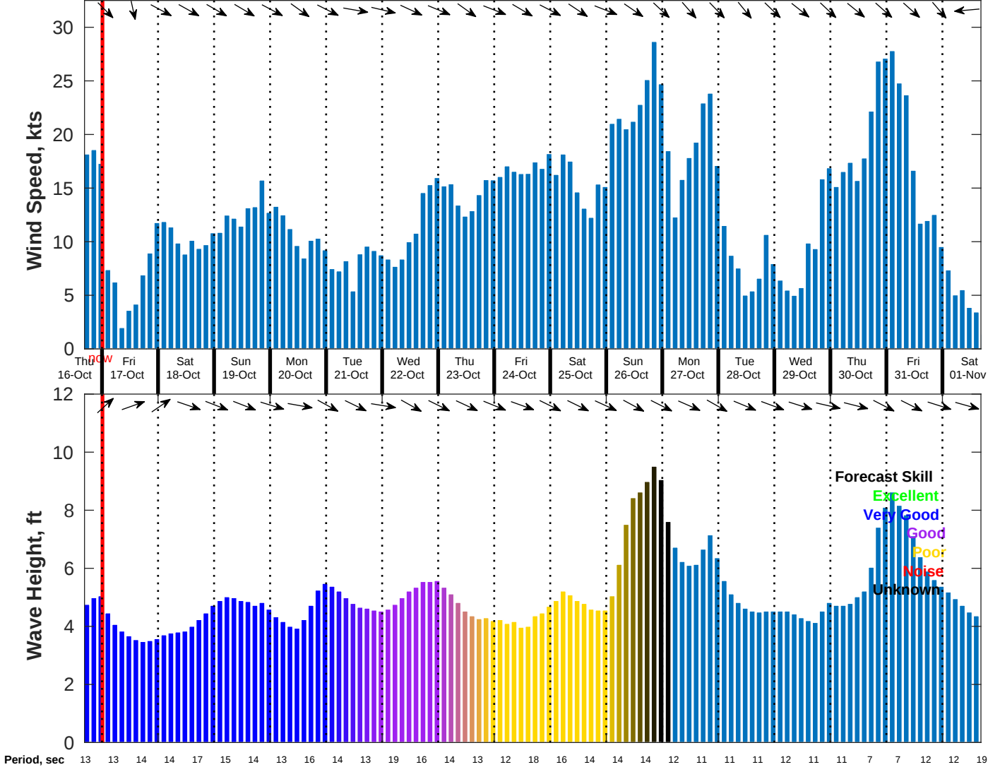
Wind & Wave Forecast for NDBC 46069 from 16-Oct-2025 16:00:00 to 01-Nov-2025 16:00:00
