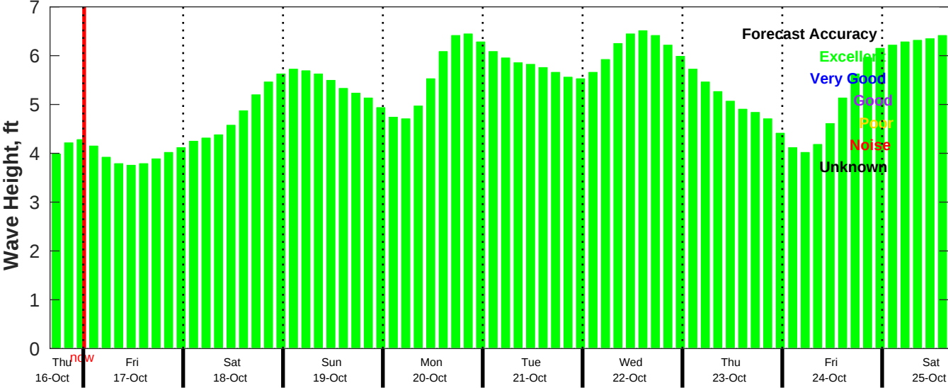
CMEMS Wave Forecast for NDBC 46215 from 16-Oct-2025 16:00:00 to 25-Oct-2025 16:00:00
