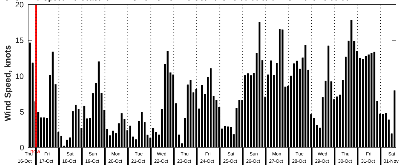
GFS Wind Speed Forecast for NDBC 46215 from 16-Oct-2025 16:00:00 to 01-Nov-2025 16:00:00
