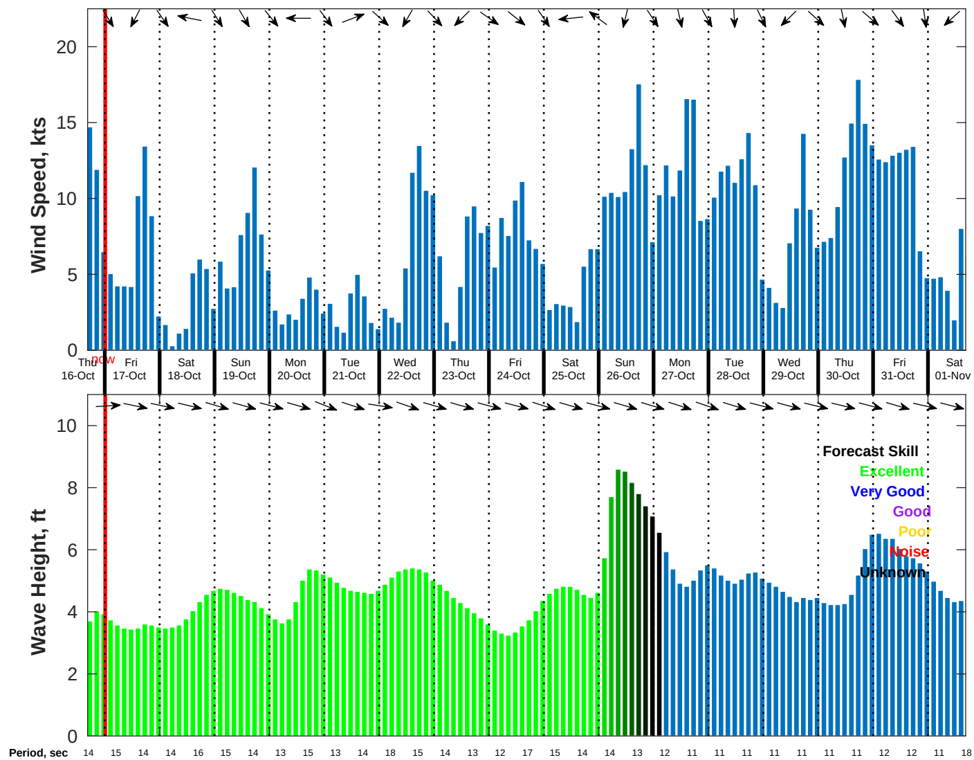
Wind & Wave Forecast for NDBC 46215 from 16-Oct-2025 16:00:00 to 01-Nov-2025 16:00:00
