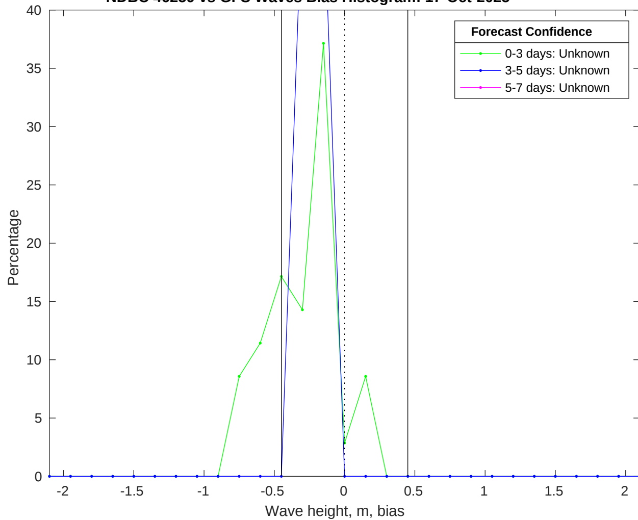
NDBC 46259 vs GFS Waves Bias Histogram: 17-Oct-2025
