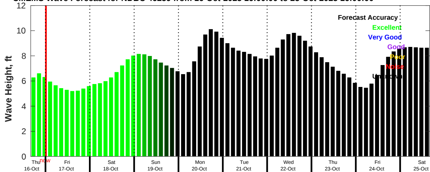
CMEMS Wave Forecast for NDBC 46259 from 16-Oct-2025 16:00:00 to 25-Oct-2025 16:00:00
