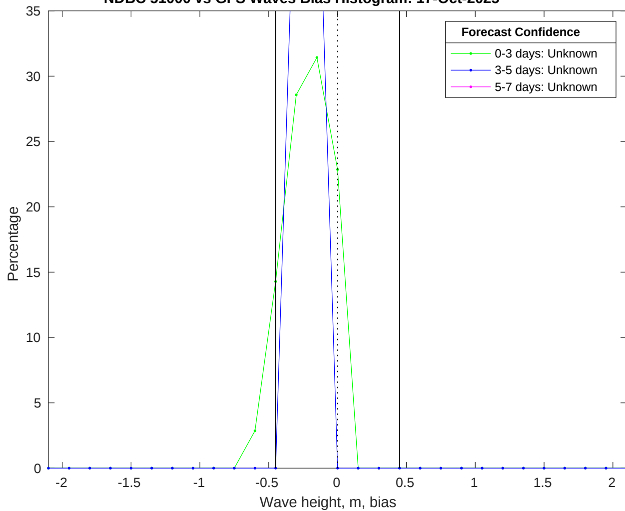
NDBC 51000 vs GFS Waves Bias Histogram: 17-Oct-2025
