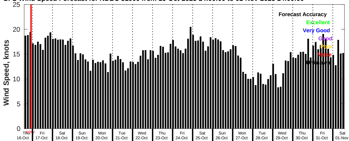
GFS Wind Speed Forecast for NDBC 51000 from 16-Oct-2025 14:00:00 to 01-Nov-2025 14:00:00
