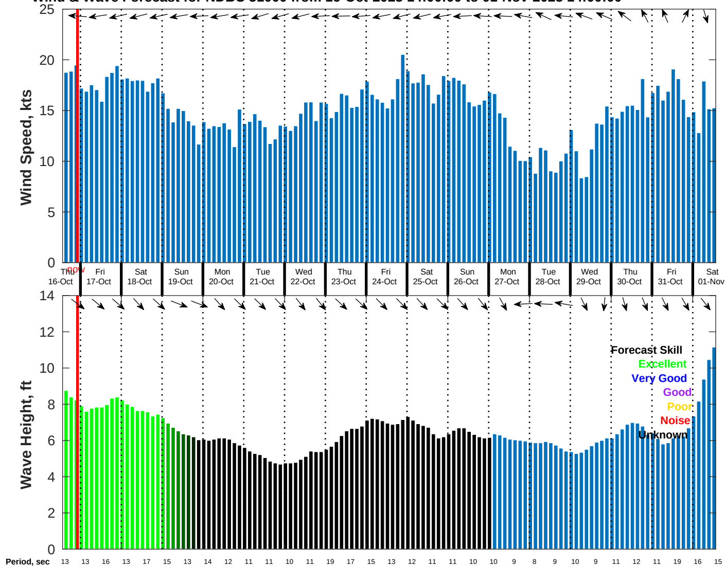
Wind & Wave Forecast for NDBC 51000 from 16-Oct-2025 14:00:00 to 01-Nov-2025 14:00:00
