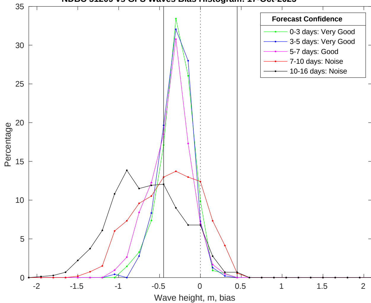
NDBC 51209 vs GFS Waves Bias Histogram: 17-Oct-2025
