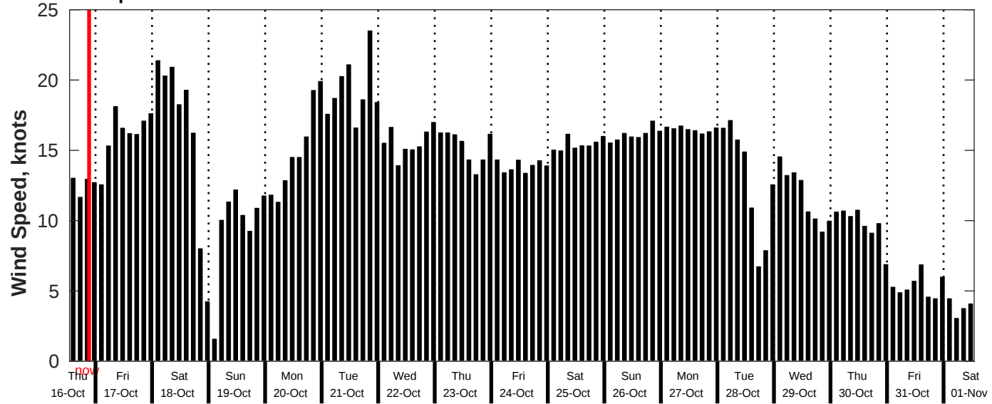
GFS Wind Speed Forecast for NDBC 51209 from 16-Oct-2025 13:00:00 to 01-Nov-2025 13:00:00
