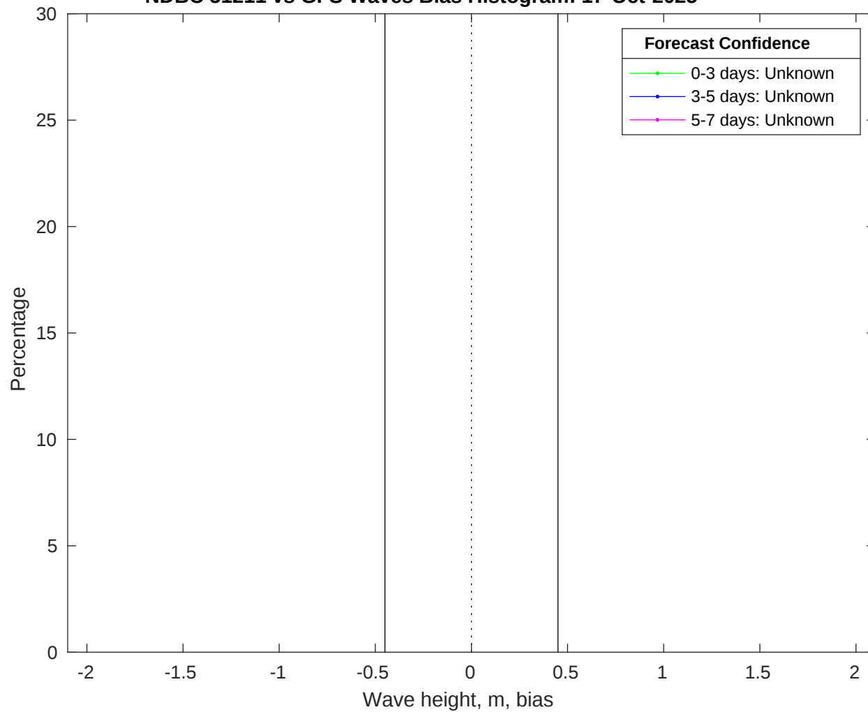
NDBC 51211 vs GFS Waves Bias Histogram: 17-Oct-2025
