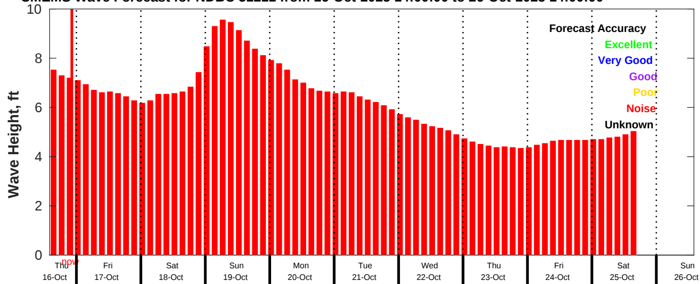
CMEMS Wave Forecast for NDBC 51211 from 16-Oct-2025 14:00:00 to 26-Oct-2025 14:00:00
