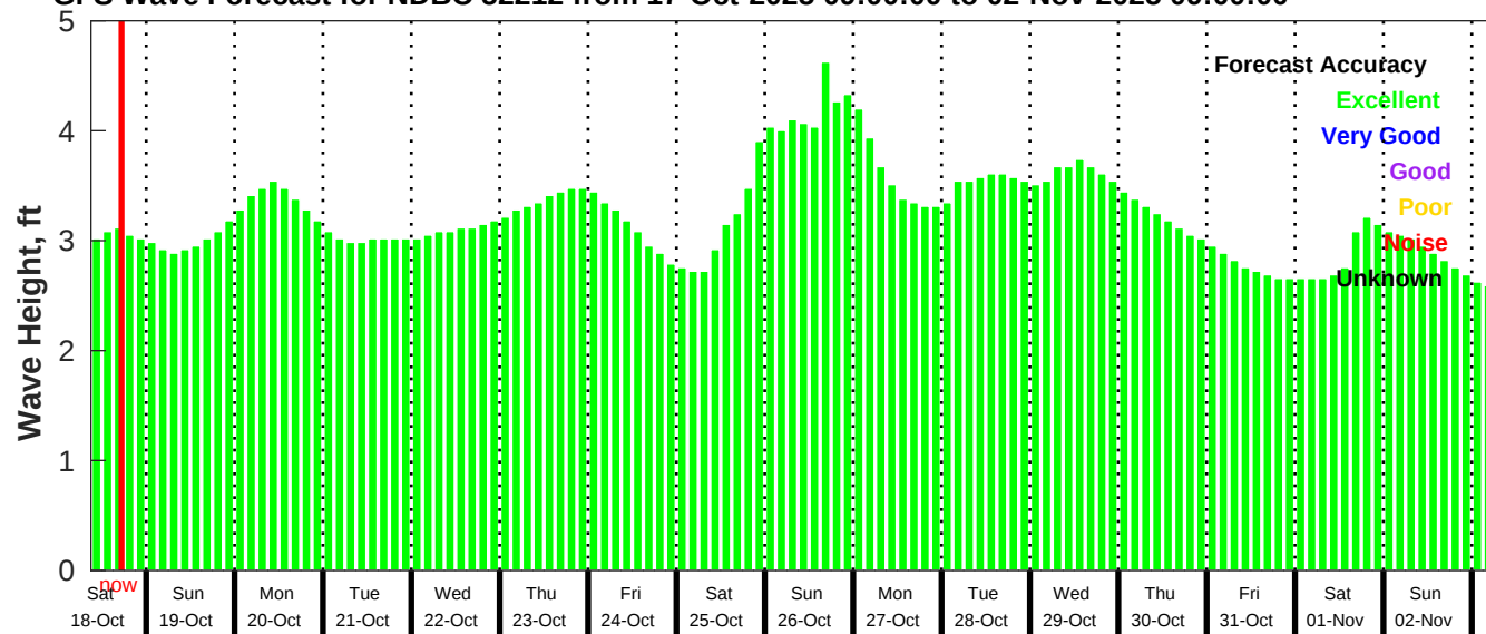
GFS Wave Forecast for NDBC 52212 from 17-Oct-2025 09:00:00 to 02-Nov-2025 09:00:00
