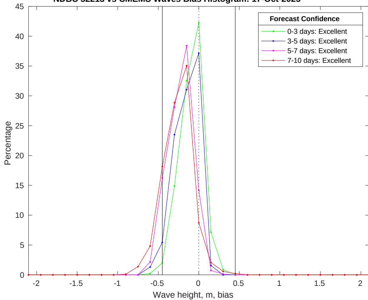
NDBC 52213 vs CMEMS Waves Bias Histogram: 17-Oct-2025
