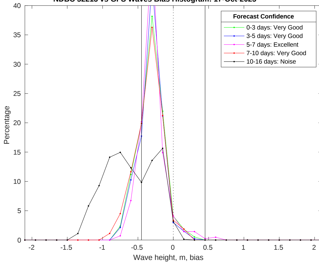
NDBC 52213 vs GFS Waves Bias Histogram: 17-Oct-2025
