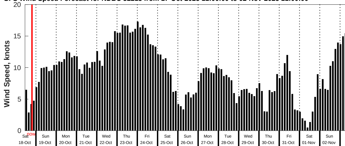
GFS Wind Speed Forecast for NDBC 52213 from 17-Oct-2025 11:00:00 to 02-Nov-2025 11:00:00
