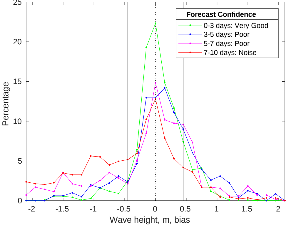
NDBC 41004 vs CMEMS Waves Bias Histogram: 16-Oct-2025
