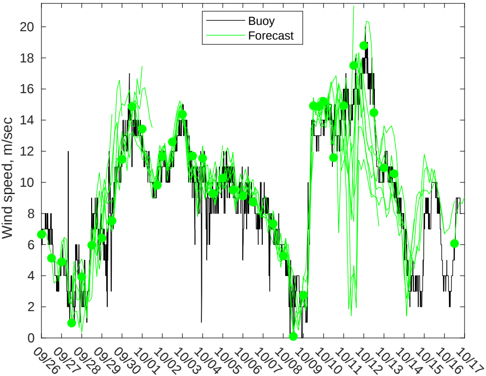
NDBC 41004 vs GFS Winds: 0 to 3 day forecast
