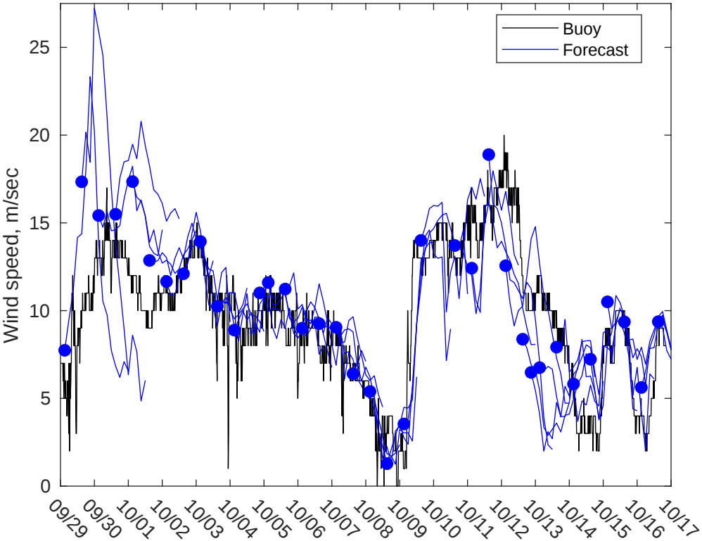
NDBC 41004 vs GFS Winds: 3 to 5 day forecast
