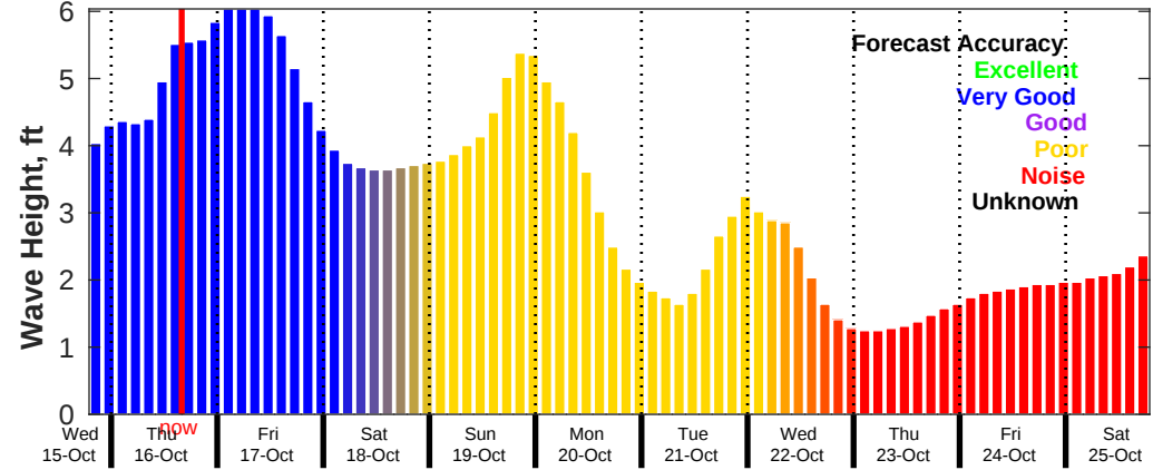
CMEMS Wave Forecast for NDBC 41004 from 15-Oct-2025 19:00:00 to 25-Oct-2025 19:00:00
