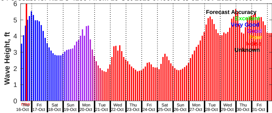
GFS Wave Forecast for NDBC 41004 from 16-Oct-2025 07:00:00 to 01-Nov-2025 07:00:00
