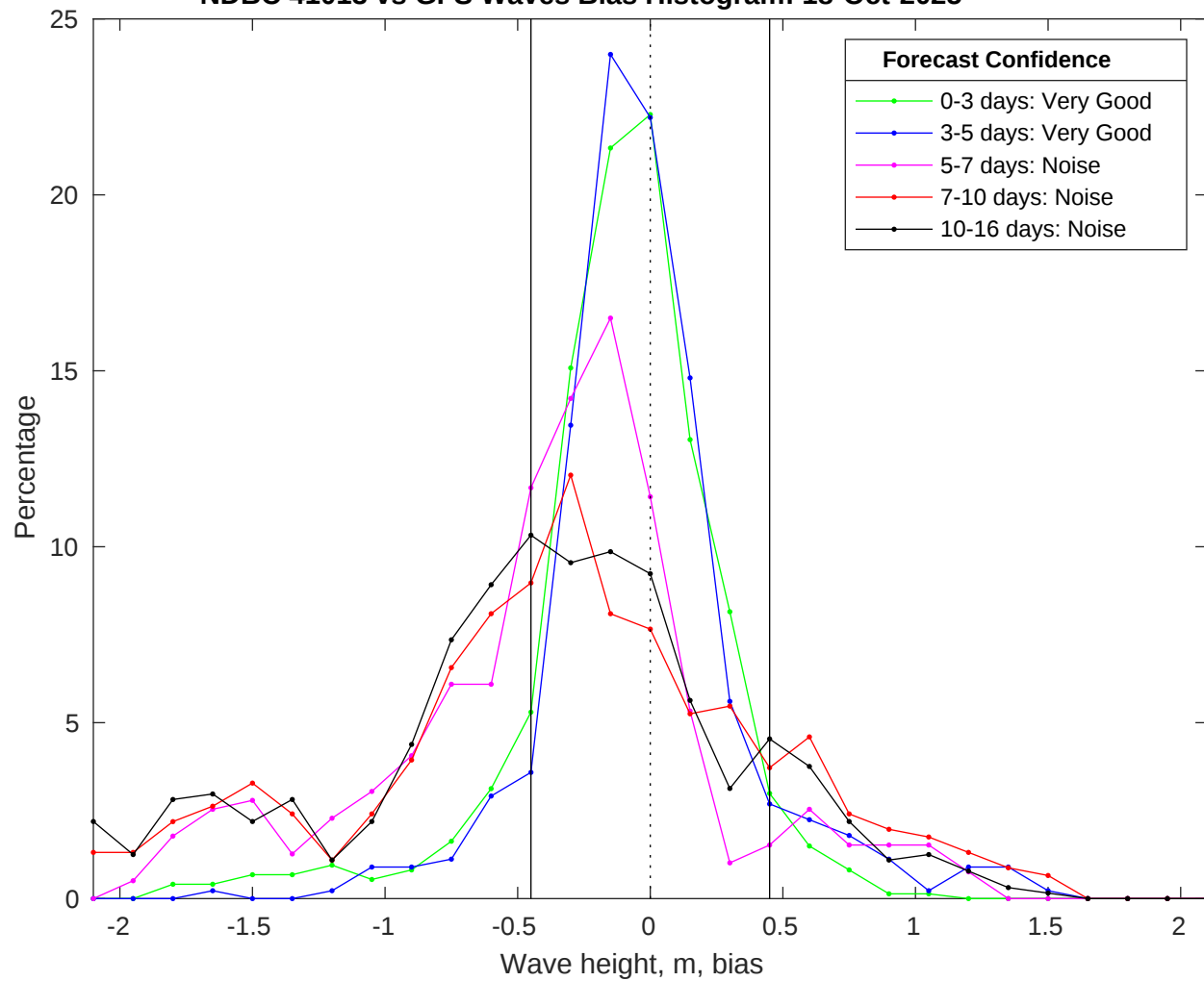
NDBC 41013 vs GFS Waves Bias Histogram: 18-Oct-2025
