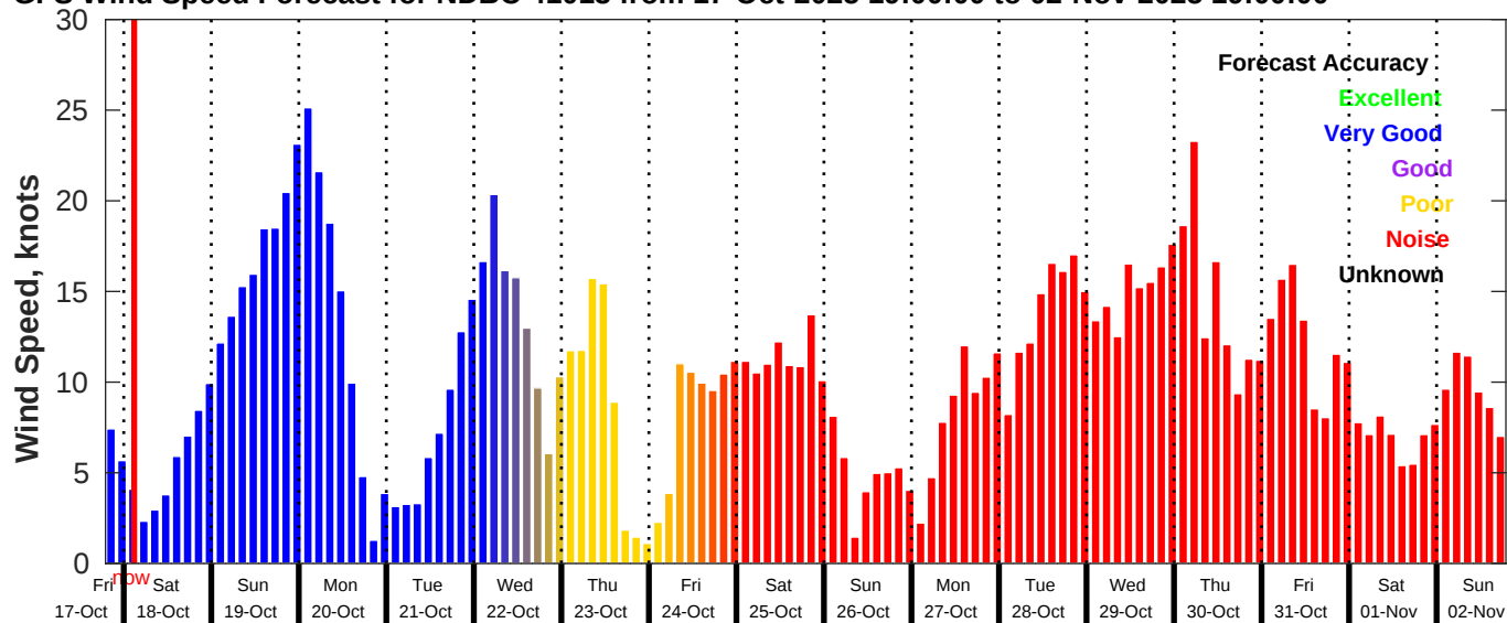
GFS Wind Speed Forecast for NDBC 41013 from 17-Oct-2025 19:00:00 to 02-Nov-2025 19:00:00
