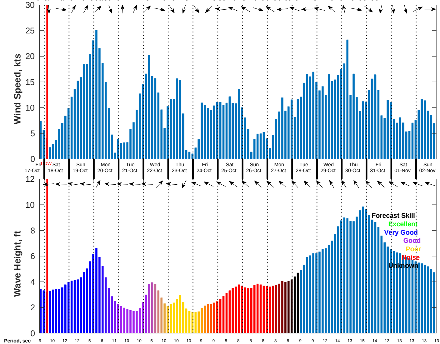
Wind & Wave Forecast for NDBC 41013 from 17-Oct-2025 19:00:00 to 02-Nov-2025 19:00:00
