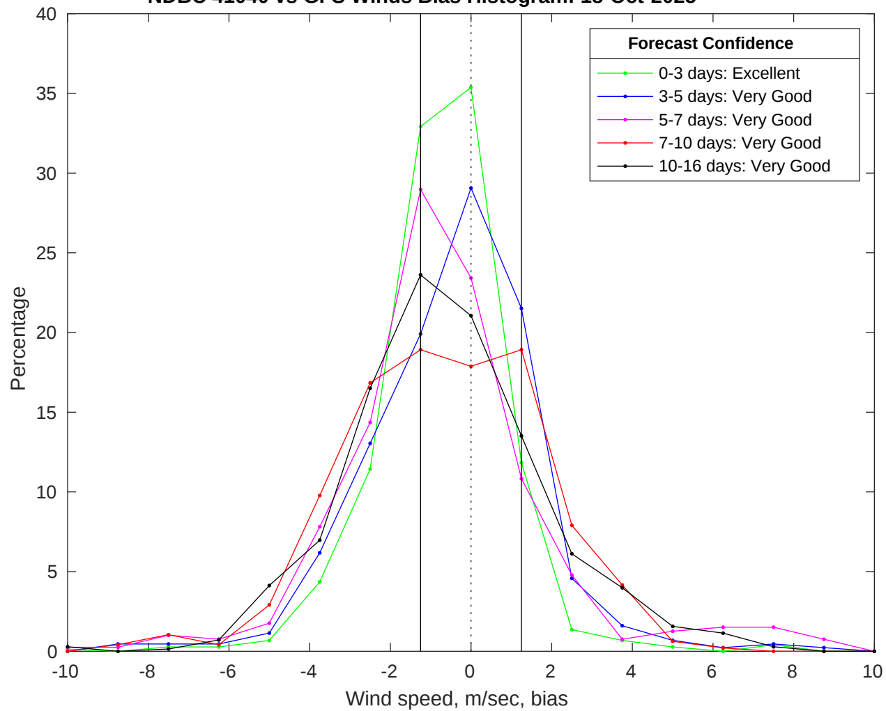
NDBC 41040 vs GFS Winds Bias Histogram: 18-Oct-2025
