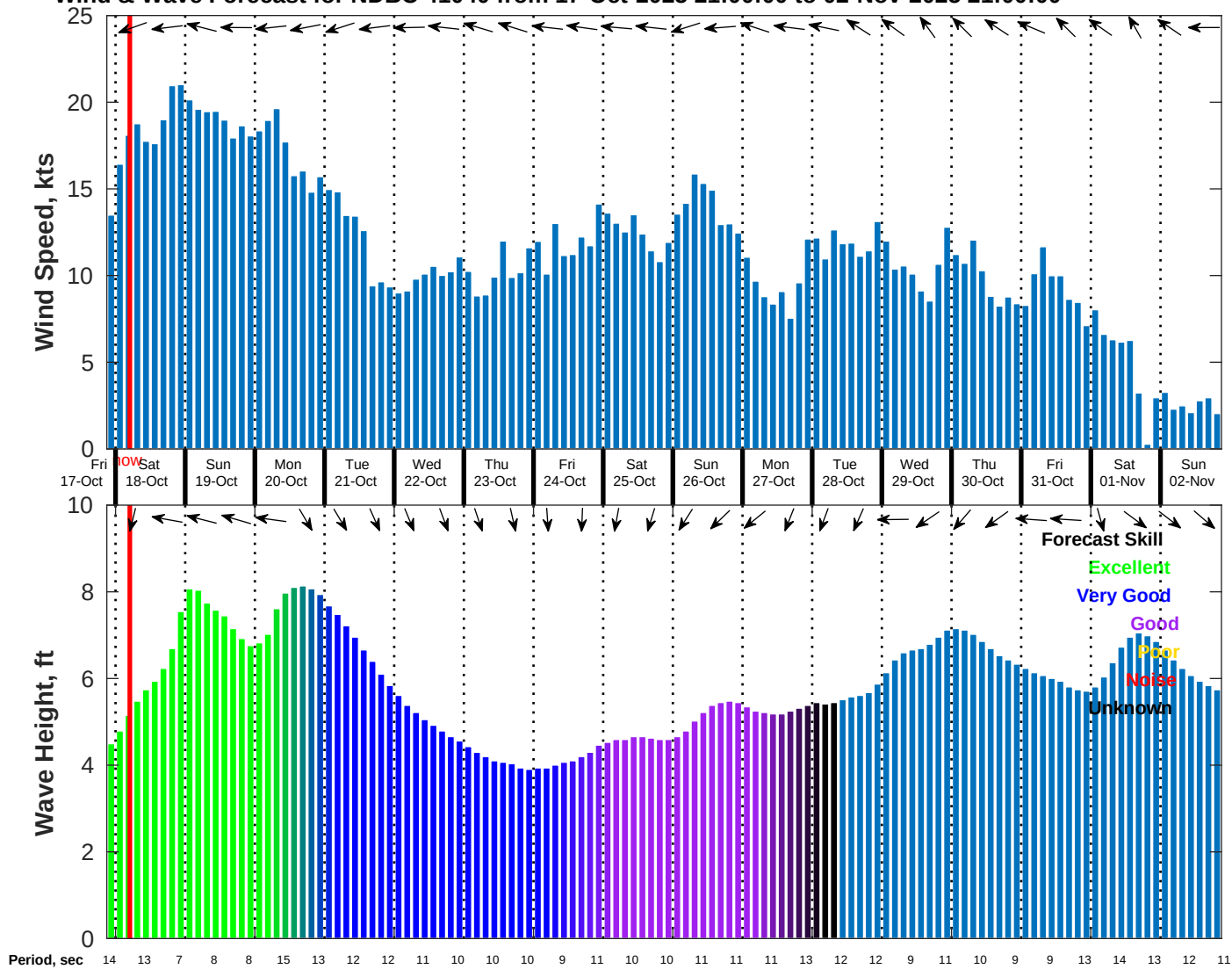
Wind & Wave Forecast for NDBC 41040 from 17-Oct-2025 21:00:00 to 02-Nov-2025 21:00:00
