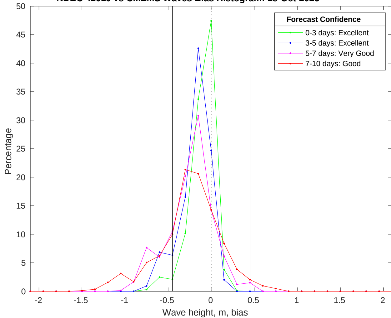
NDBC 42019 vs CMEMS Waves Bias Histogram: 18-Oct-2025
