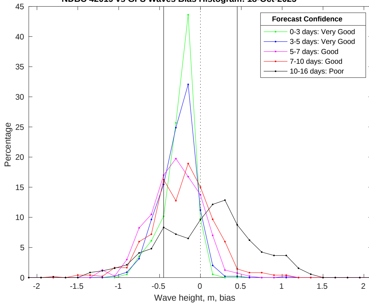
NDBC 42019 vs GFS Waves Bias Histogram: 18-Oct-2025
