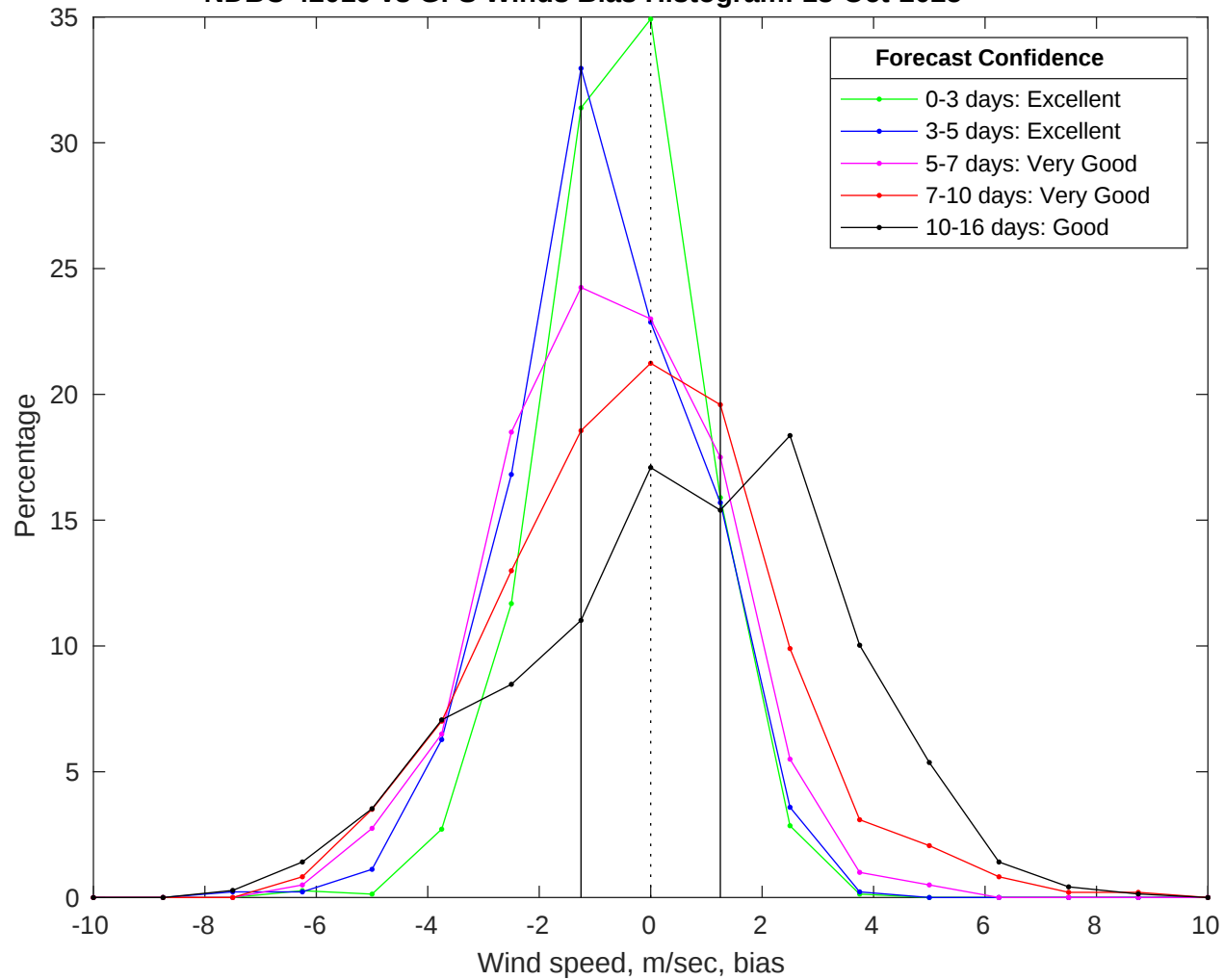
NDBC 42019 vs GFS Winds Bias Histogram: 18-Oct-2025
