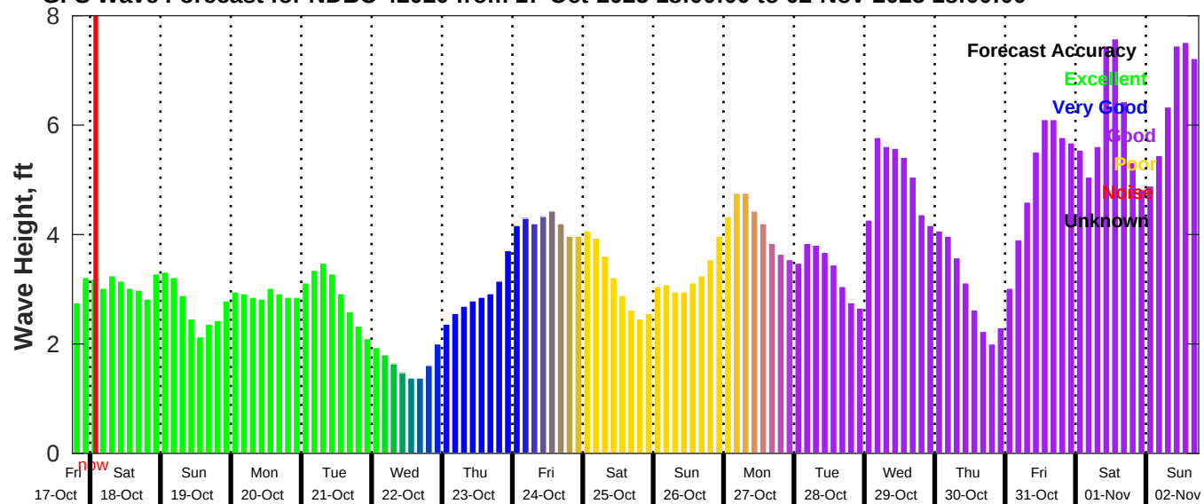
GFS Wave Forecast for NDBC 42020 from 17-Oct-2025 18:00:00 to 02-Nov-2025 18:00:00
