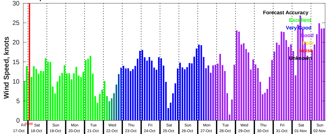
GFS Wind Speed Forecast for NDBC 42020 from 17-Oct-2025 18:00:00 to 02-Nov-2025 18:00:00
