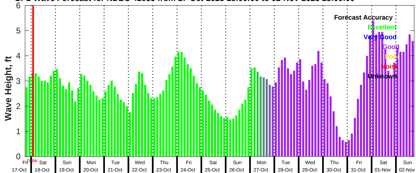
GFS Wave Forecast for NDBC 42035 from 17-Oct-2025 18:00:00 to 02-Nov-2025 18:00:00
