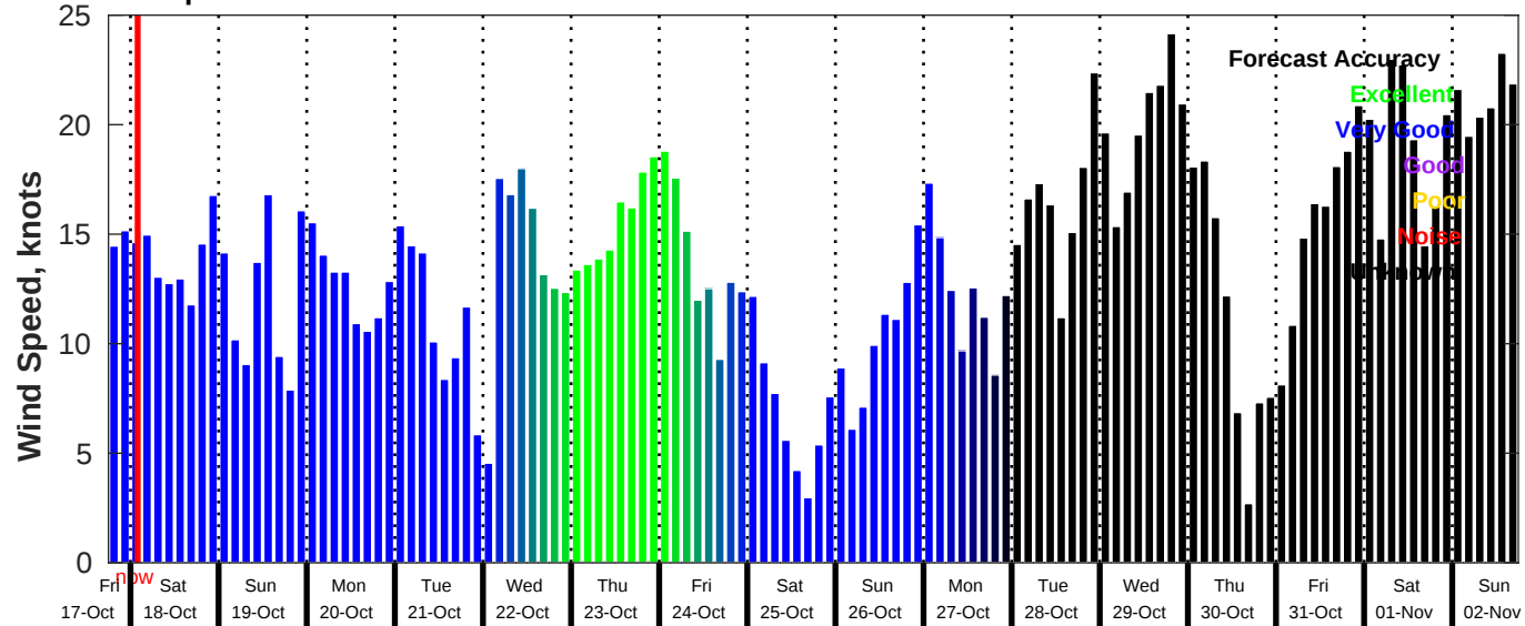
GFS Wind Speed Forecast for NDBC 42035 from 17-Oct-2025 18:00:00 to 02-Nov-2025 18:00:00
