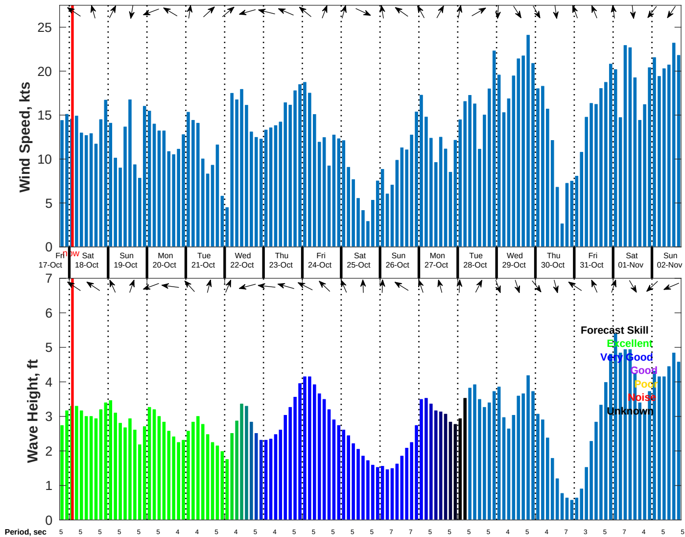
Wind & Wave Forecast for NDBC 42035 from 17-Oct-2025 18:00:00 to 02-Nov-2025 18:00:00
