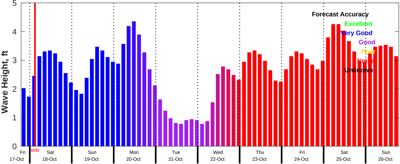
CMEMS Wave Forecast for NDBC 42036 from 17-Oct-2025 19:00:00 to 26-Oct-2025 19:00:00
