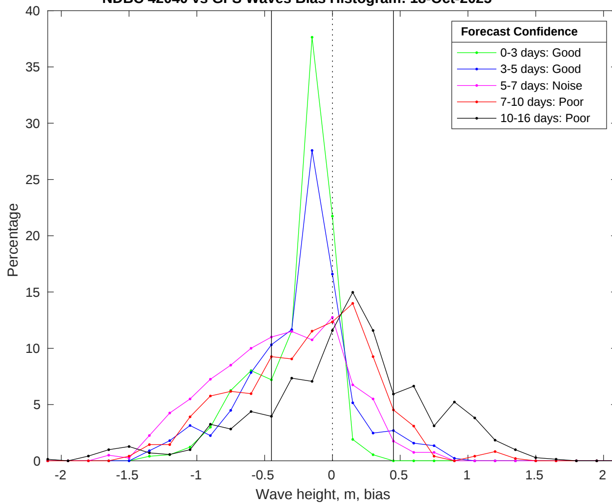
NDBC 42040 vs GFS Waves Bias Histogram: 18-Oct-2025
