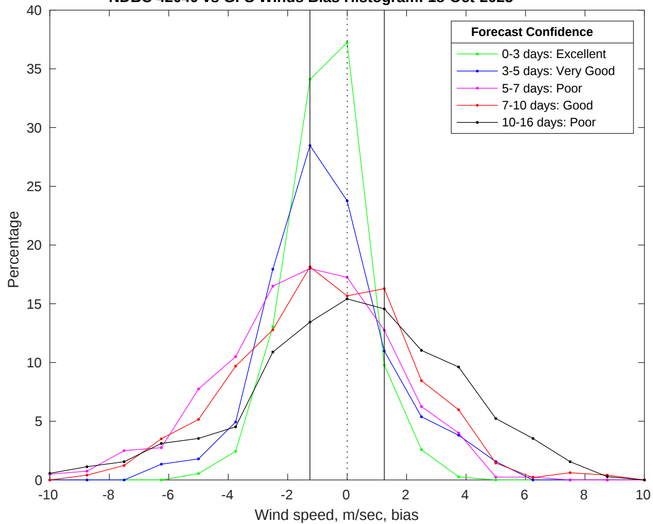
NDBC 42040 vs GFS Winds Bias Histogram: 18-Oct-2025
