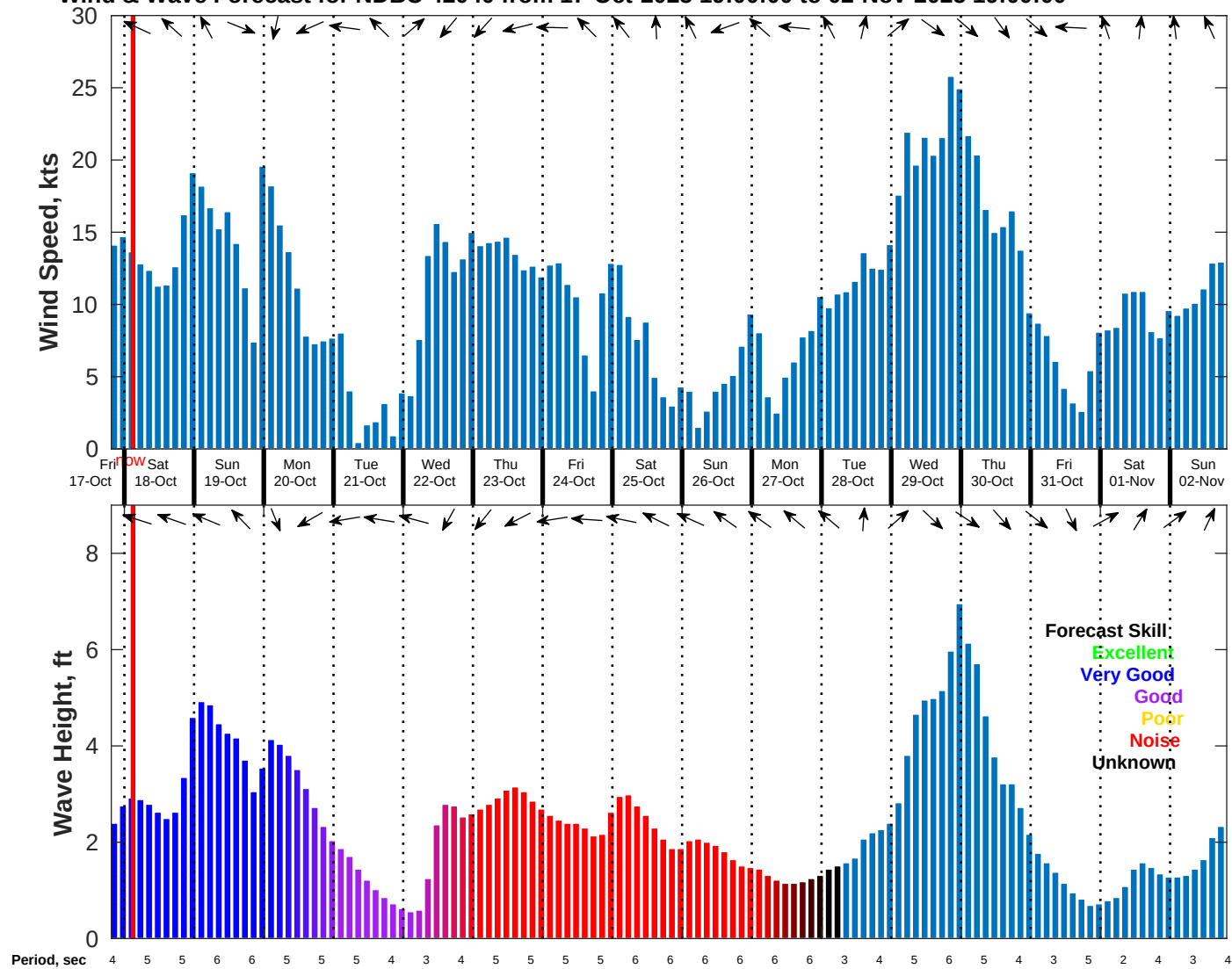
Wind & Wave Forecast for NDBC 42040 from 17-Oct-2025 19:00:00 to 02-Nov-2025 19:00:00
