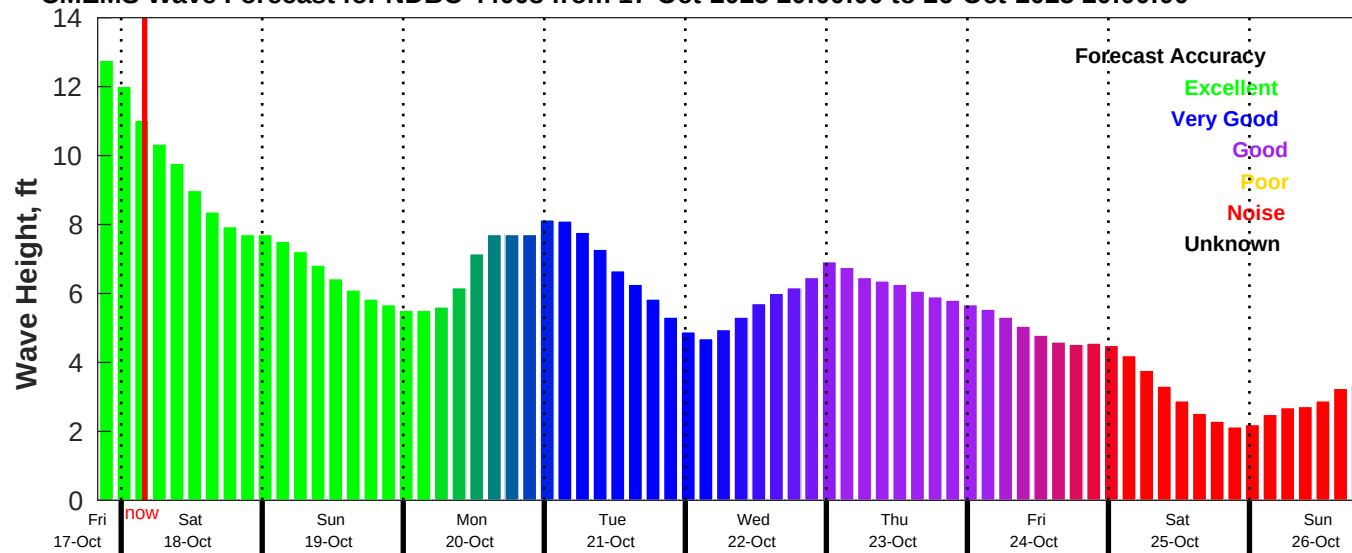
CMEMS Wave Forecast for NDBC 44008 from 17-Oct-2025 20:00:00 to 26-Oct-2025 20:00:00
