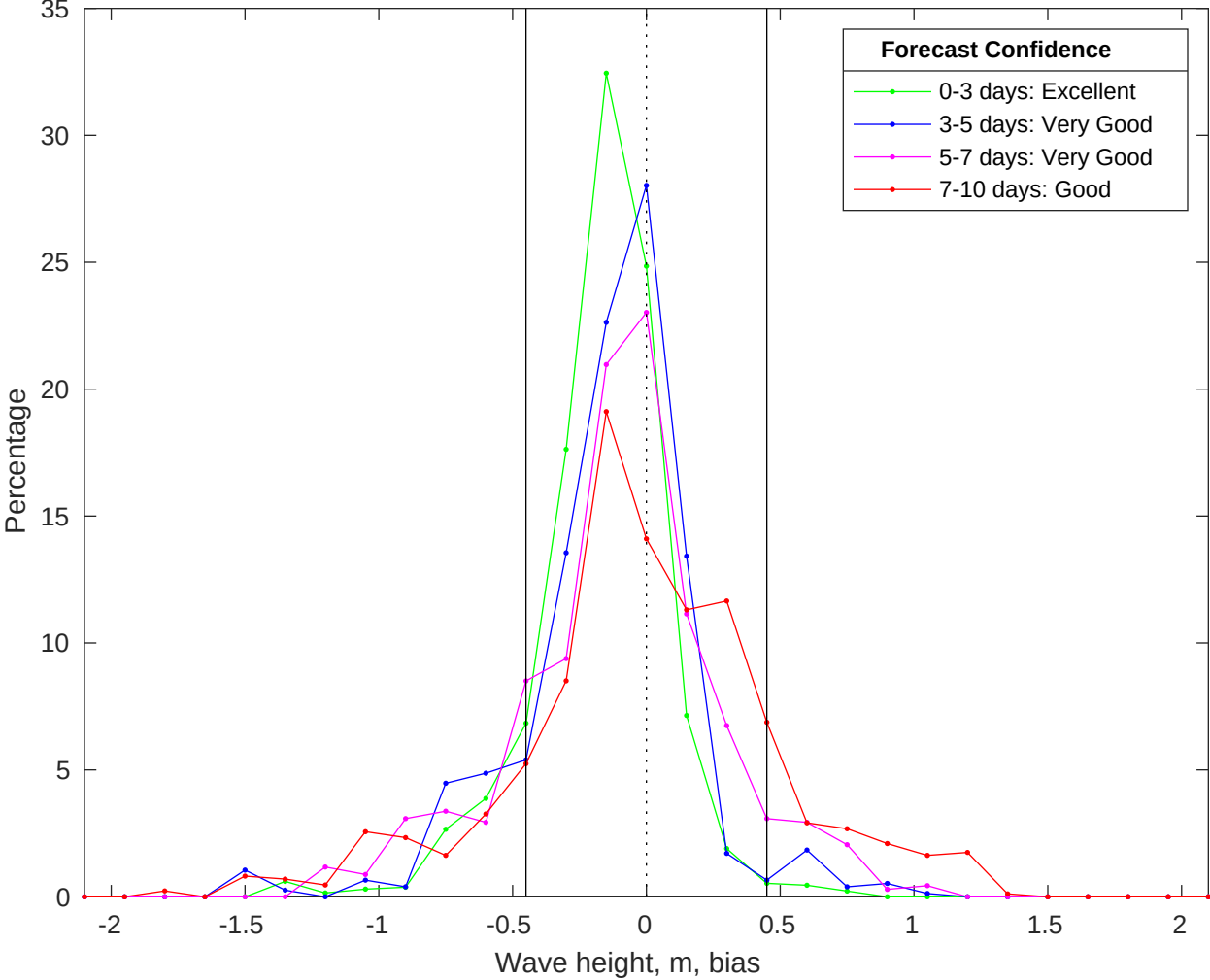
NDBC 46028 vs CMEMS Waves Bias Histogram: 18-Oct-2025
