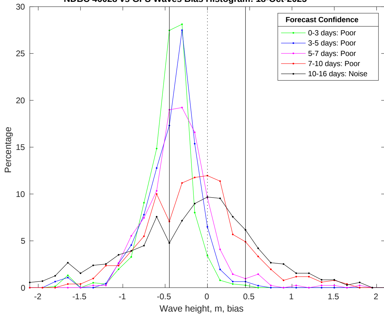
NDBC 46028 vs GFS Waves Bias Histogram: 18-Oct-2025
