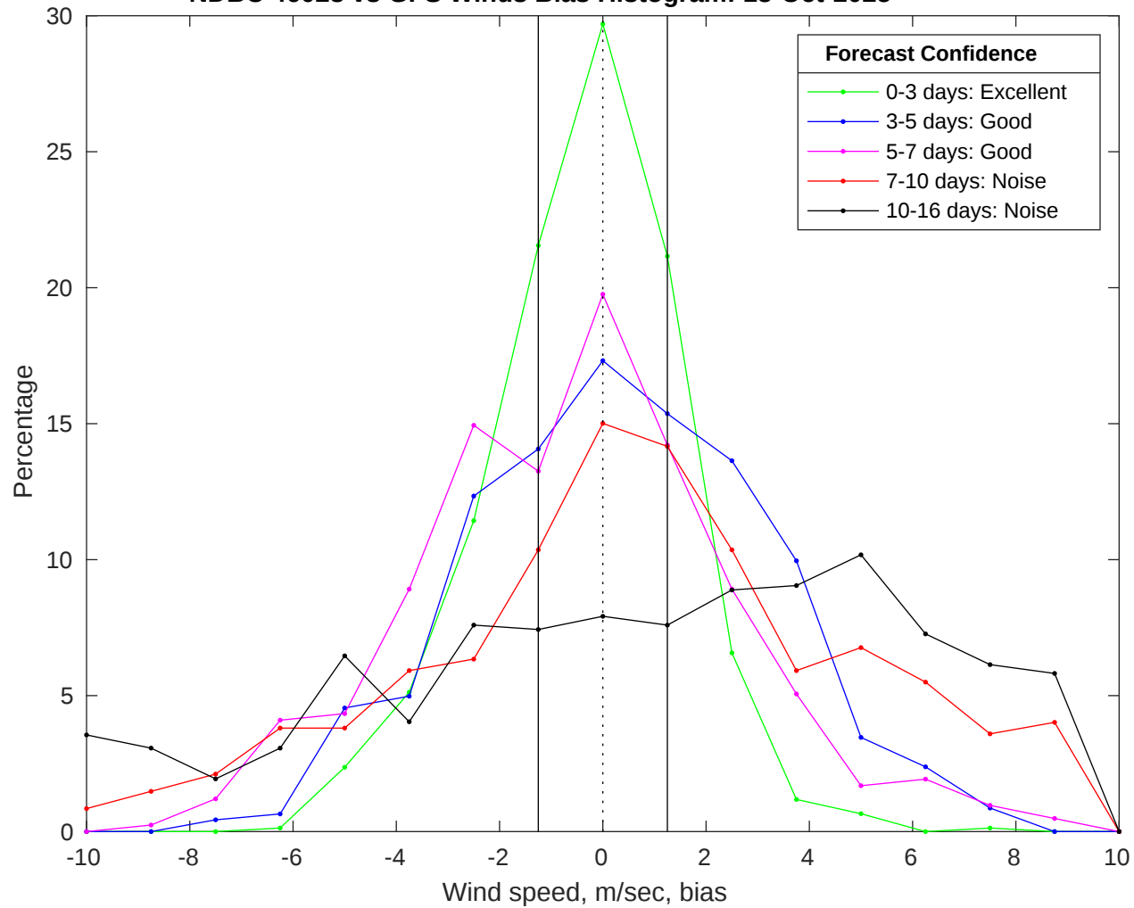
NDBC 46028 vs GFS Winds Bias Histogram: 18-Oct-2025
